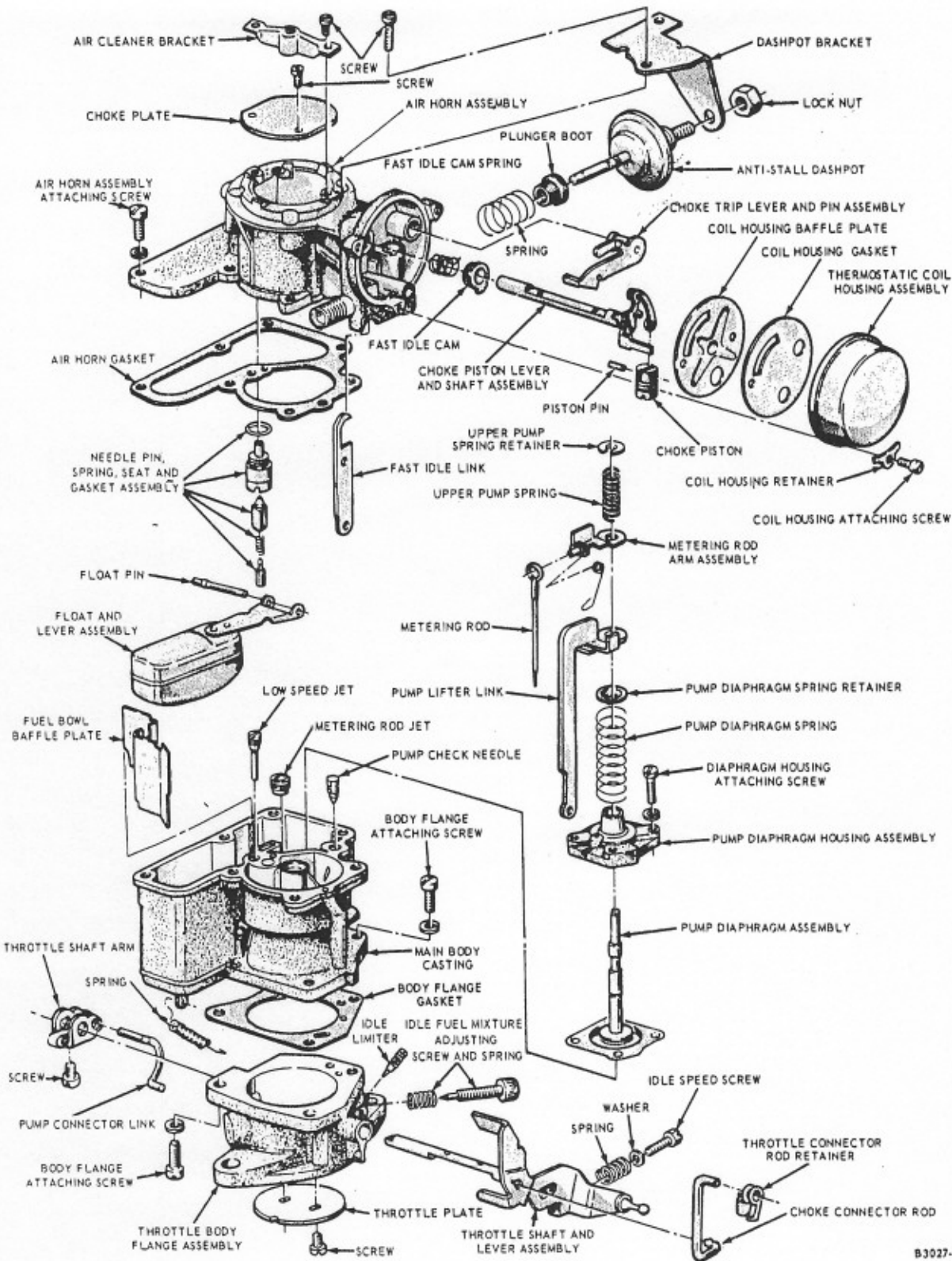
FIG. 11—Carter Model YF Carburetor Assembly
