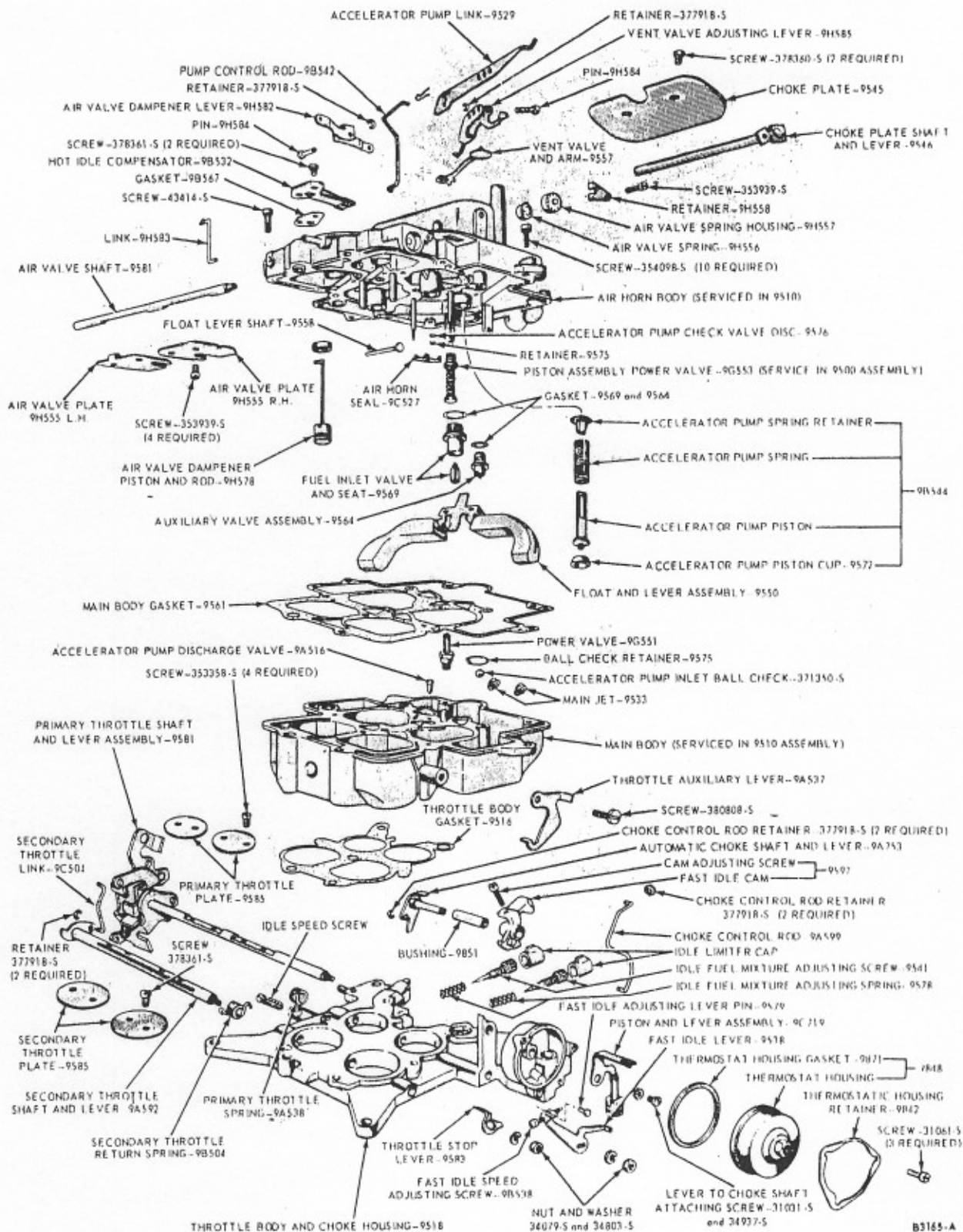
FIG. 14—Carburetor Assembly
