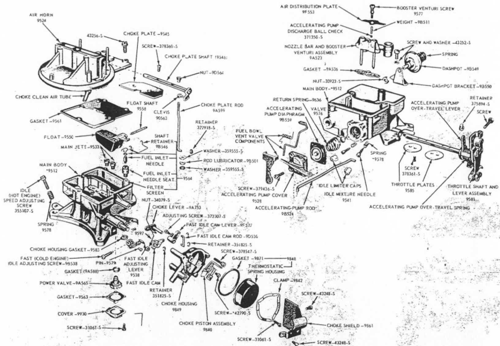
FIG. 20—Carburetor Assembly
